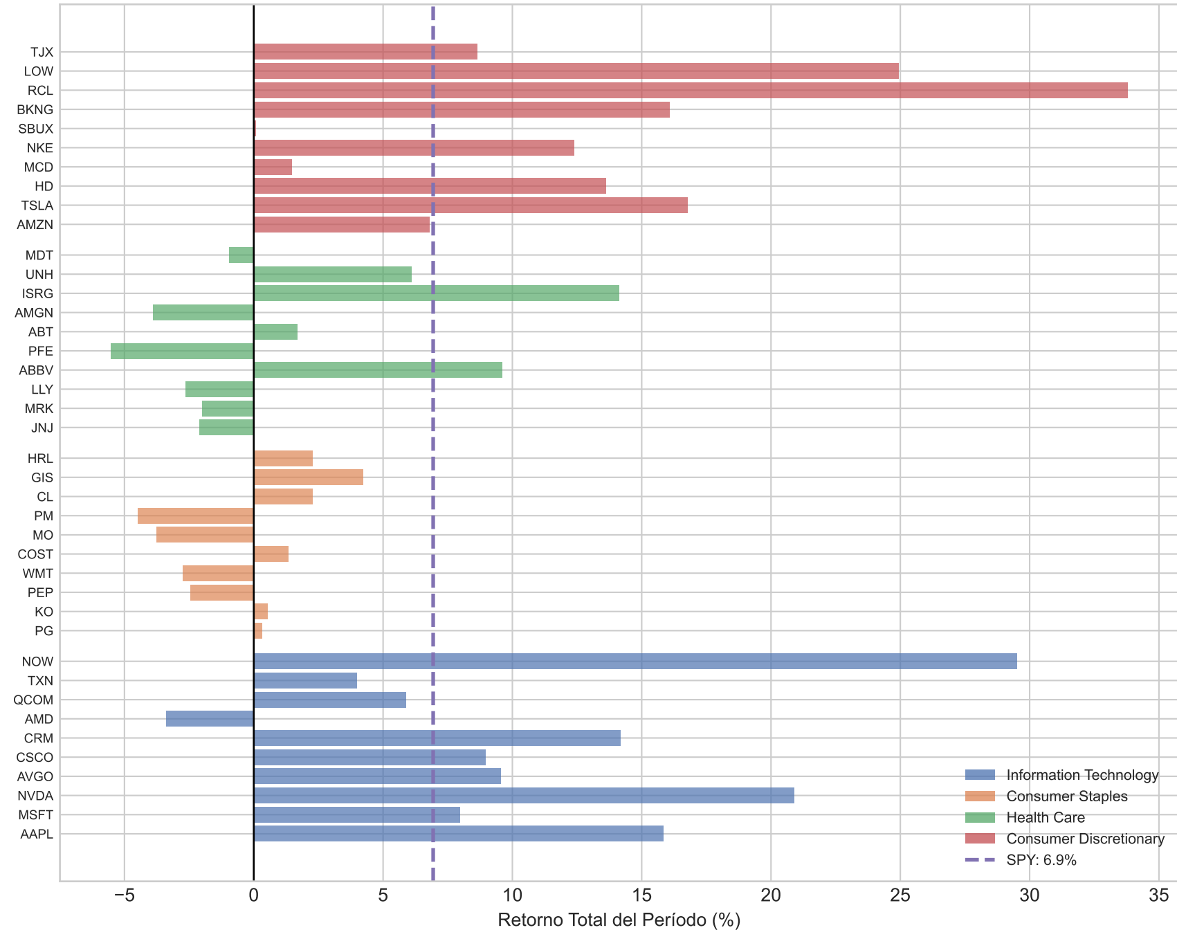
COVID-19 Crash (19 feb – 23 mar 2020)
